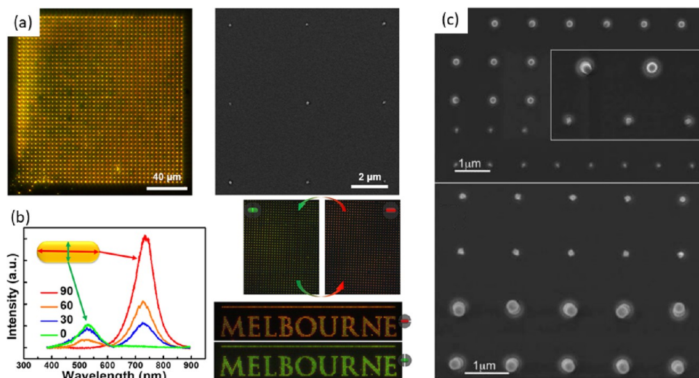
Figure 6. (a) Dark-field image of 110 nm gold nanospheres assembled by EP in a 40 \times 40 array. Inset is an SEM image of nine assembled nanospheres. Reprinted with permission from ref 130. Copyright 2018, American Chemical Society. (b) Scattering spectra of a gold nanorod at different polarization angles and dark-field images of assembled gold nanorod arrays under 0^\circ and 90^\circ polarization. Reprinted with permission from ref 130. Copyright 2018, American Chemical Society. (c) EP assembly of 200 and 100 nm PSL nanoparticles in 210 and 110 nm circles, respectively (top); EP assembly of 200 and 50 nm PSL nanoparticles in 225 and 100 nm circles (bottom). Reprinted with permission from ref 131. Copyright 2011, American Chemical Society.
