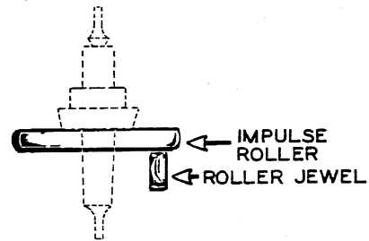
SINGLE ROLLER
