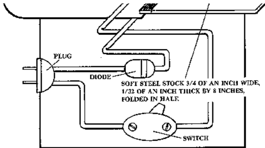
Figure 30. The magnetic pick is easy to construct.
