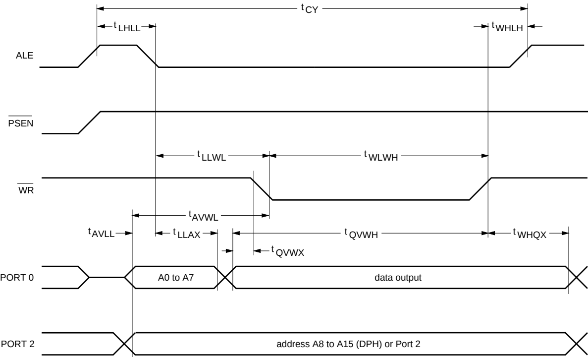
Fig.29 Write to external Data Memory.
