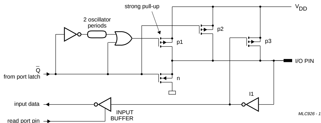
Fig.8 I/O buffers in the P8xCE560 (Port 1 to Port 4).
