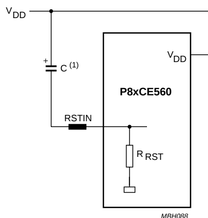
Fig.21 Power-on-reset.
