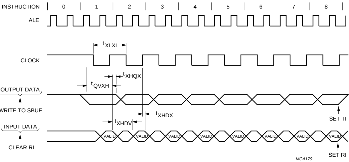
Fig.30 UART waveforms in Shift Register Mode.
