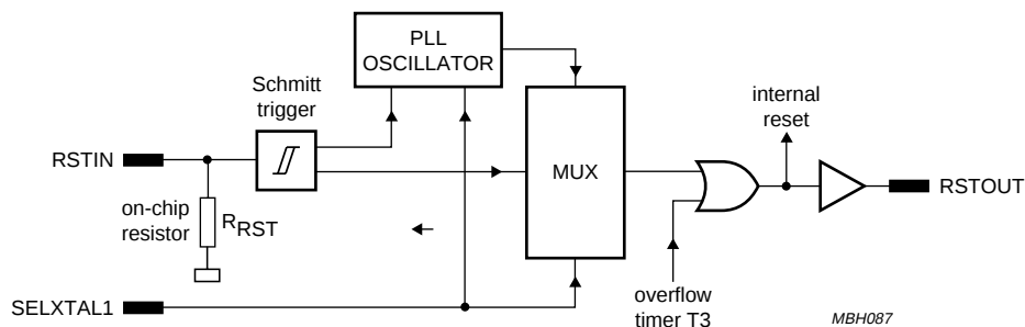
Fig.20 On-chip reset configuration.
