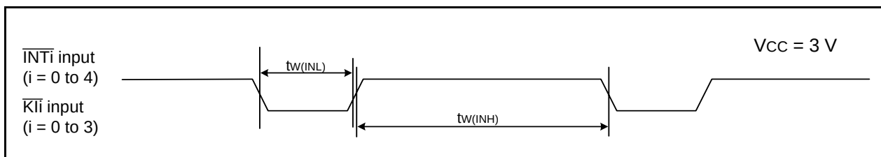
Figure 34.15 Input Timing for External Interrupt \overline{INTi} and Key Input Interrupt \overline{Kli} when Vcc = 3 V
