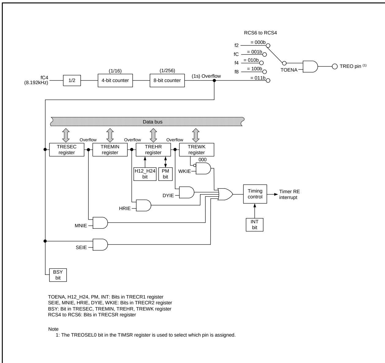
Figure 21.1 Block Diagram of Real-Time Clock Mode
