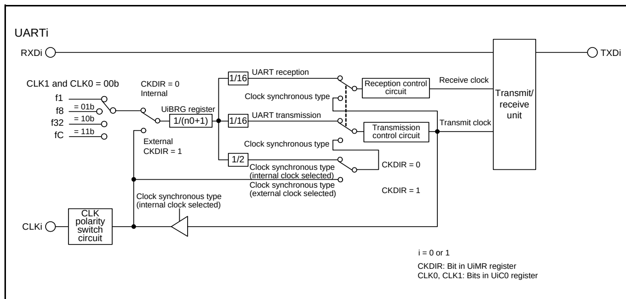
Figure 22.1 UARTi (i = 0 or 1) Block Diagram
