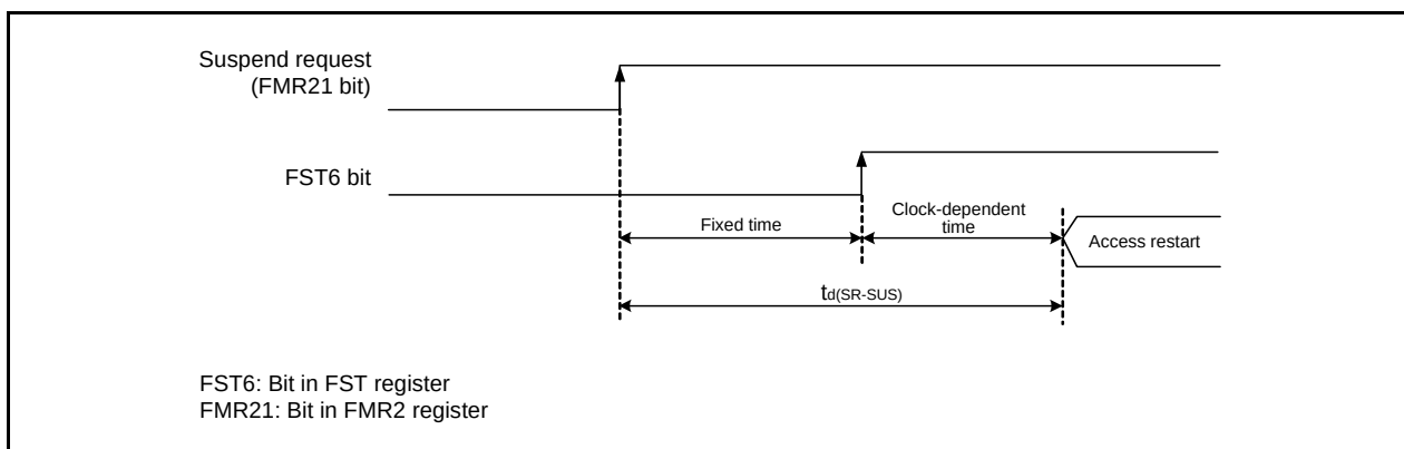
Figure 34.2 Time delay until Suspend
