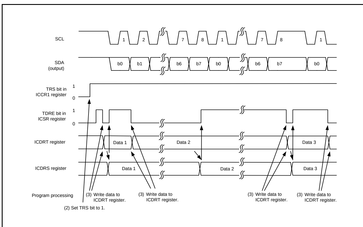
Figure 26.13 Operating Timing in Transmit Mode (Clock Synchronous Serial Mode)
