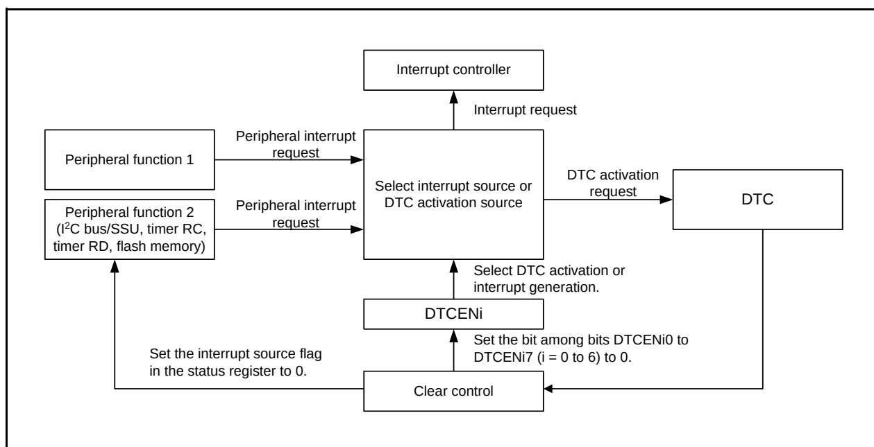
Figure 15.2 Block Diagram Showing Control of DTC Activation Sources
