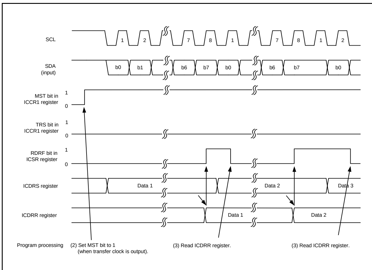
Figure 26.14 Operating Timing in Receive Mode (Clock Synchronous Serial Mode)
