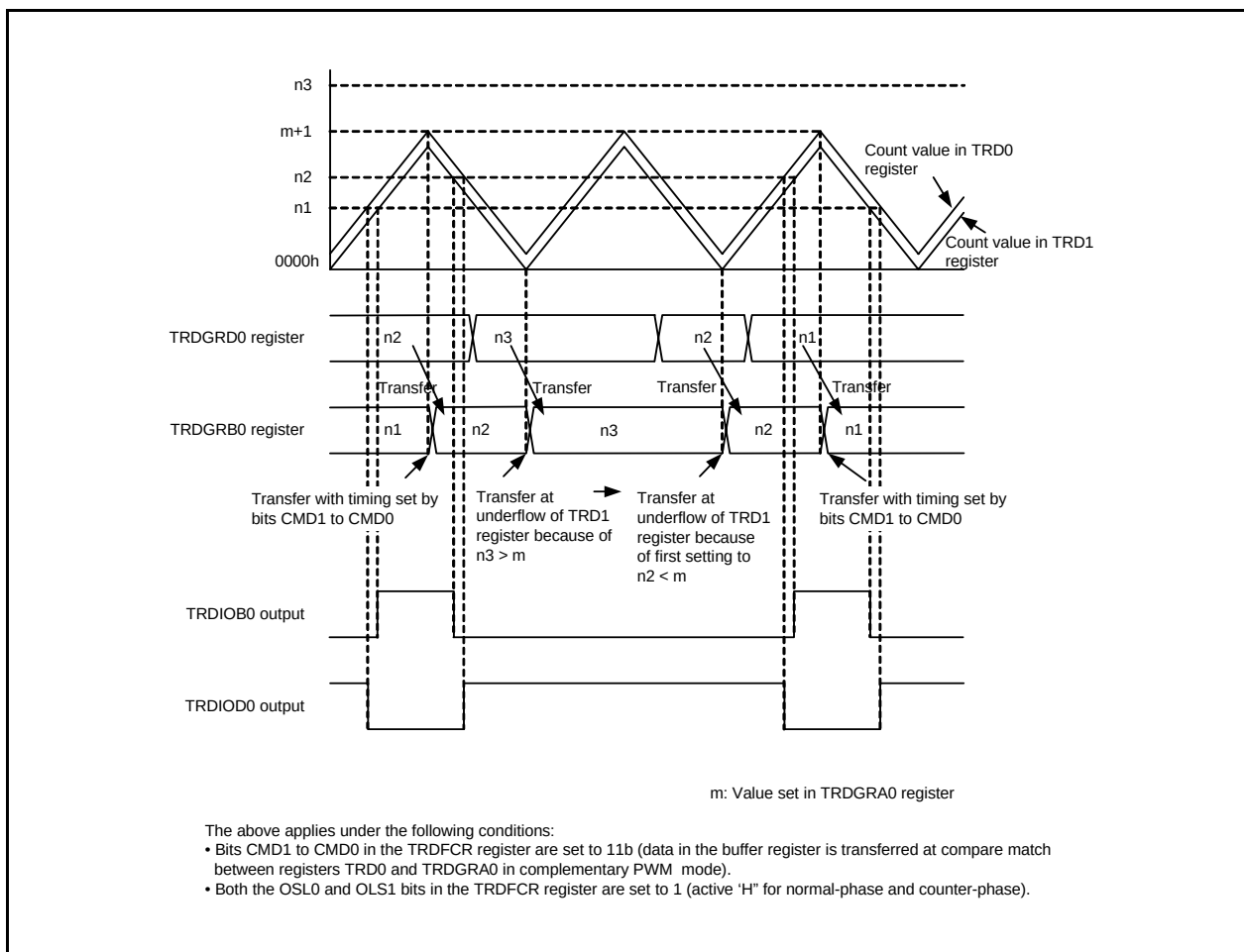
Figure 35.4 Operation when Value in Buffer Register \geq Value in TRDGRA0 Register in Complementary PWM Mode
