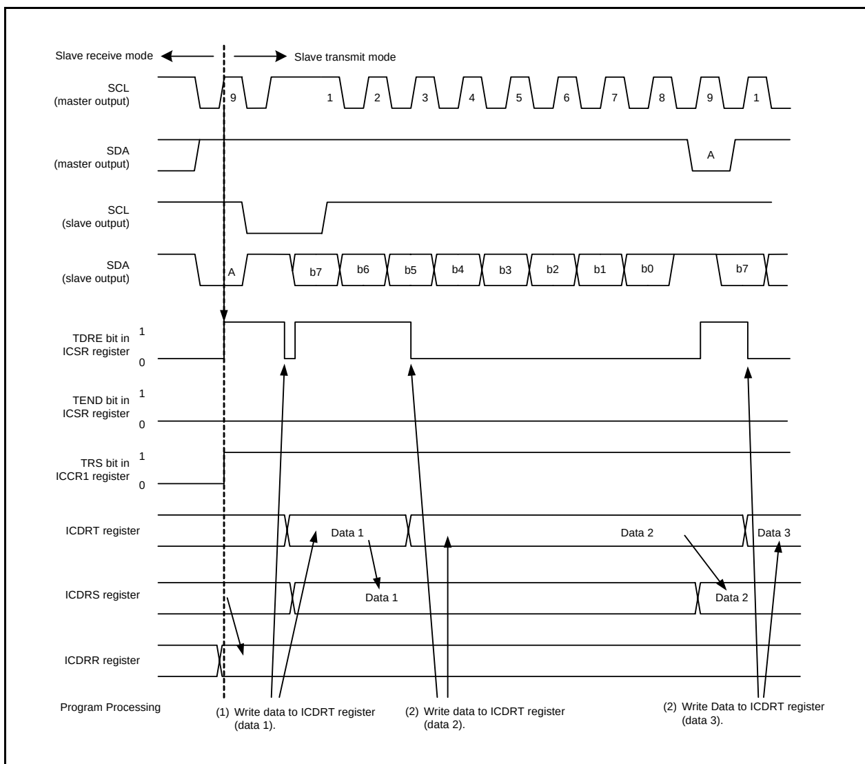
Figure 26.8 Operating Timing in Slave Transmit Mode (I 2 C bus Interface Mode) (1)
