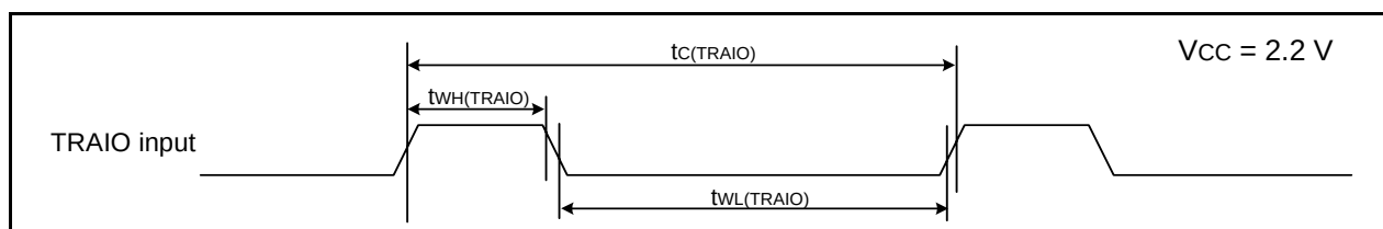
Figure 34.17 TRAIO Input Timing Diagram when V_{CC} = 2.2\text{ V}
