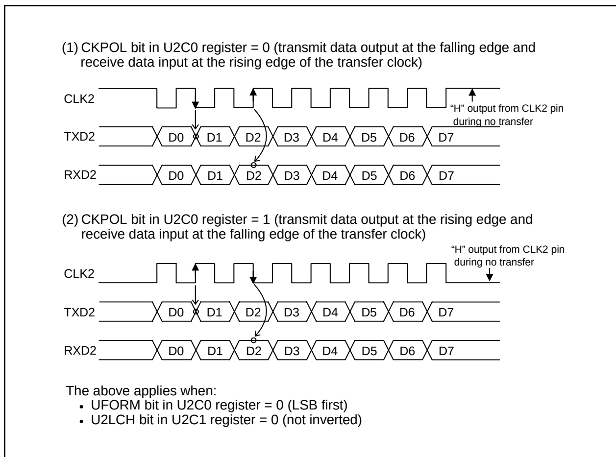
Figure 23.4 Transfer Clock Polarity
