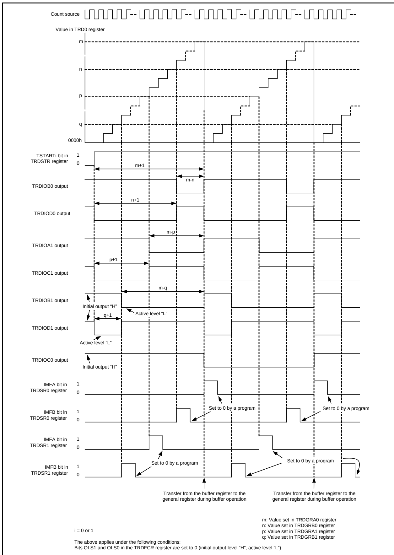
Figure 20.18 Operating Example of Reset Synchronous PWM Mode
