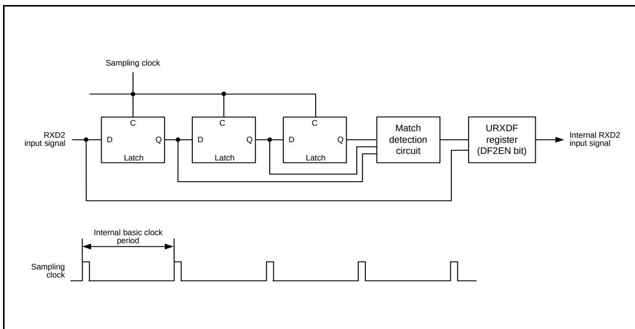
Figure 23.13 Block Diagram of RXD2 Digital Filter Circuit
