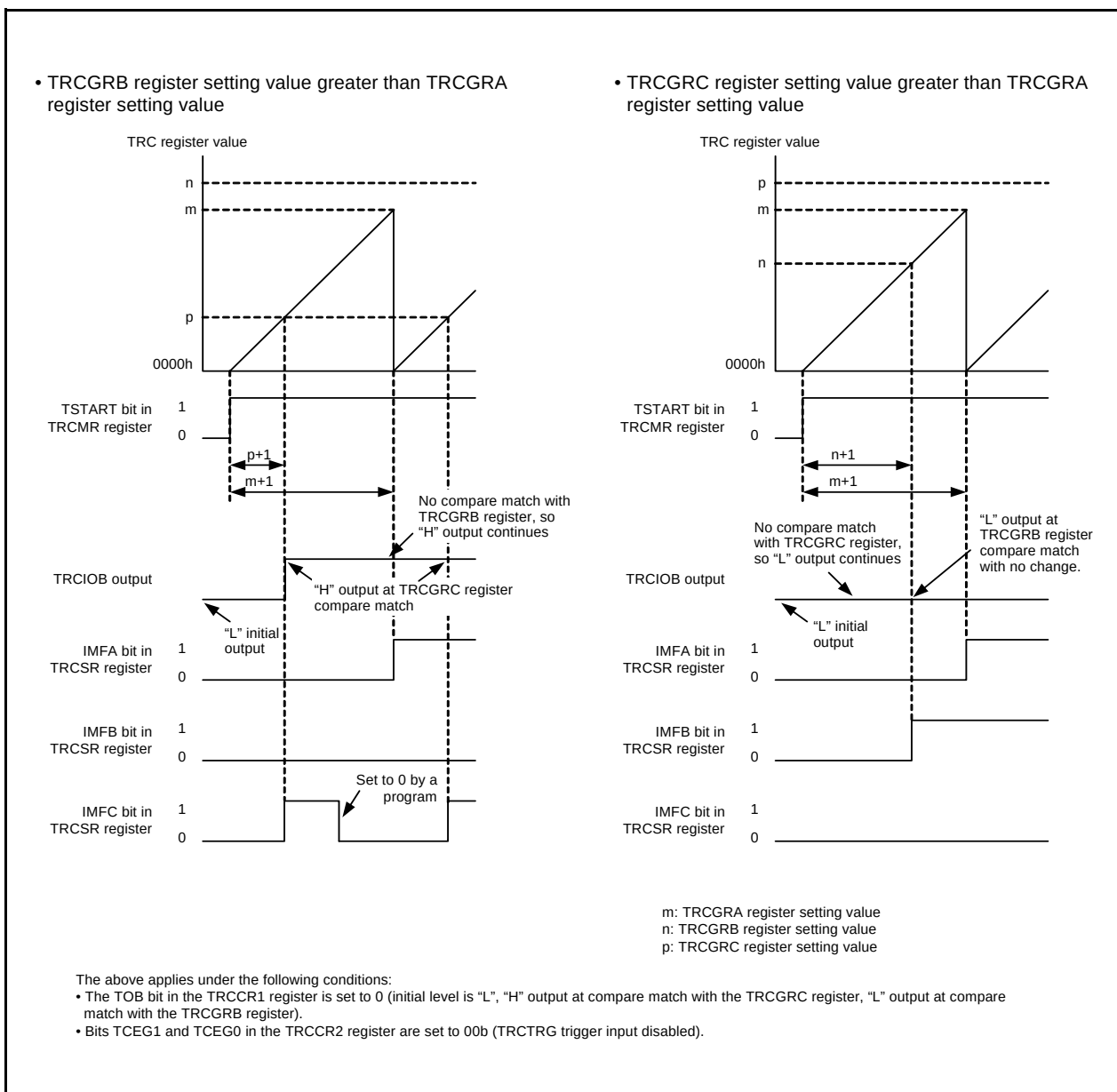
Figure 19.19 Operating Example of PWM2 Mode (Duty 0% and Duty 100%)
