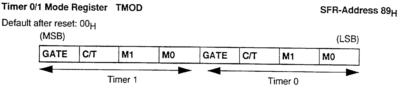
Figure 16 Timer/Counter Mode Register
