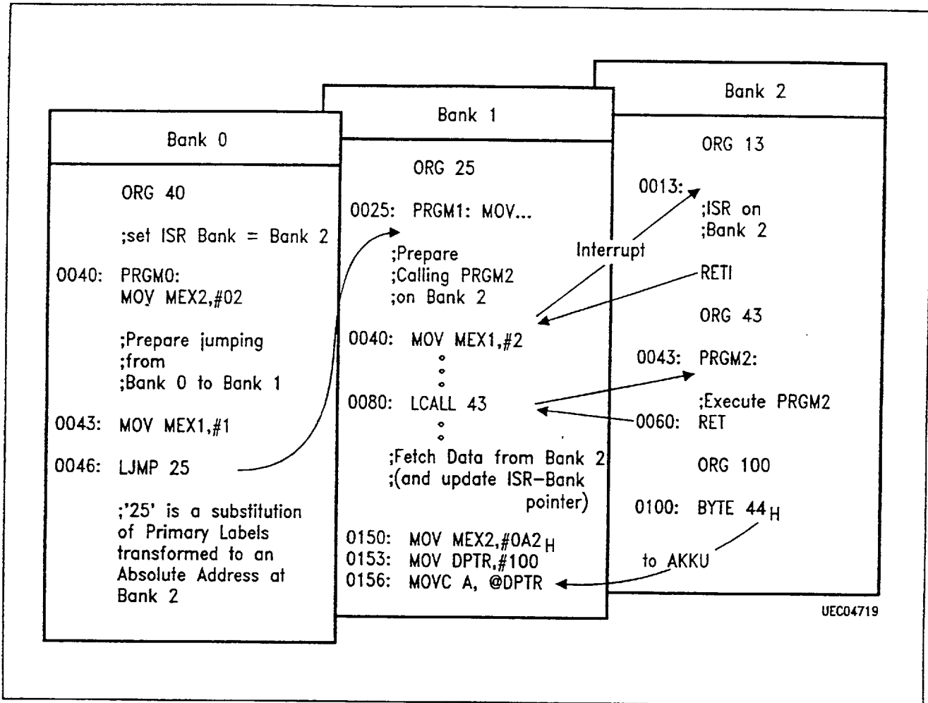
Figure 7 Program Example
