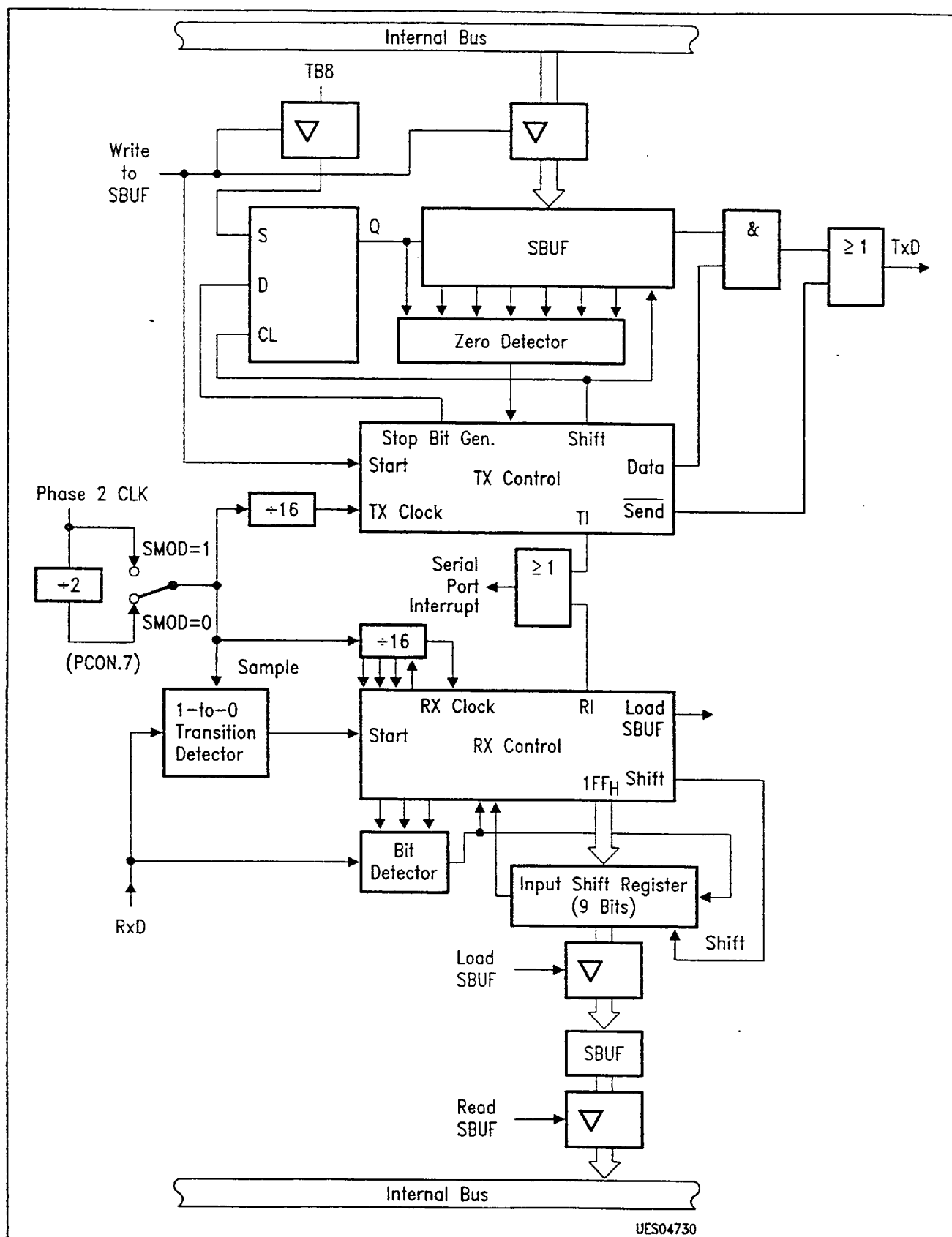
Figure 24 a Serial Port Mode 2, Functional Diagram
