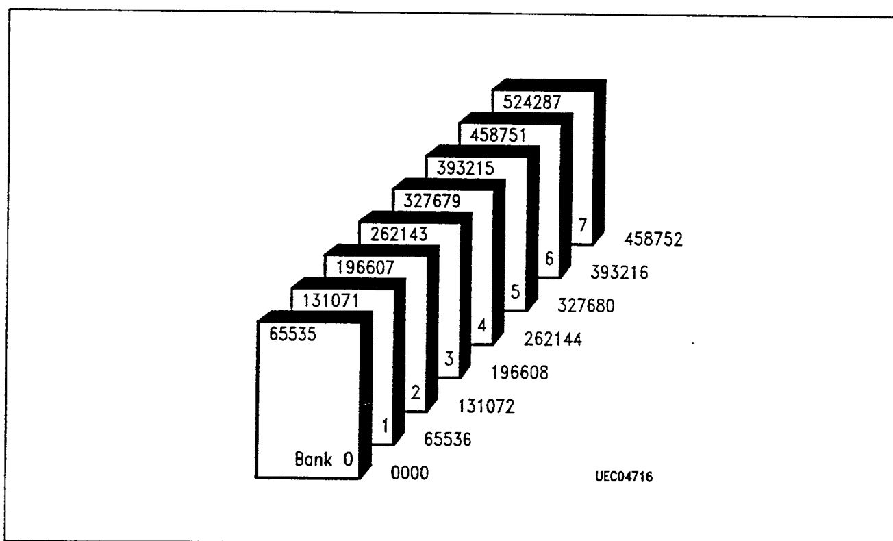
Figure 3 Bank Organization
