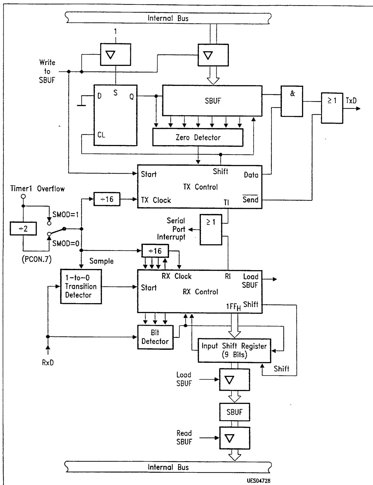
Figure 23 a Serial Port Mode 1, Functional Diagram
