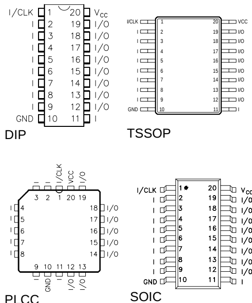
Figure 1 Pin Configuration
