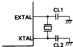
Figure 65 Crystal Interface
