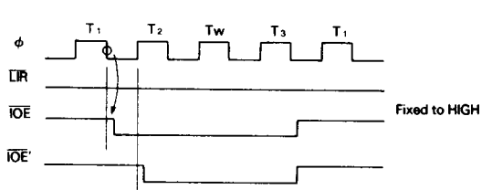
(b) I/O Read/Write Timing
