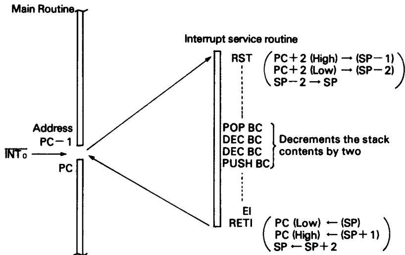
(a) \overline{\text{INT}}_0 Mode 0 Sequence when executing RST
