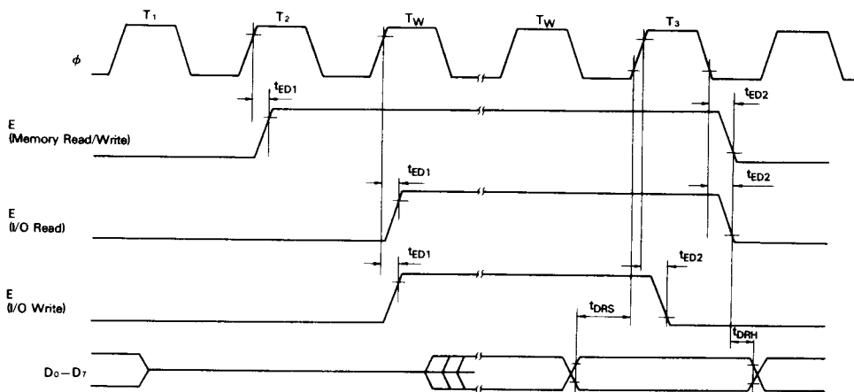
Figure 3 E Clock Timing (1)
