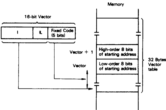
Figure 29 \overline{INT_1} , \overline{INT_2} and Internal Interrupts Vector Acquisition
