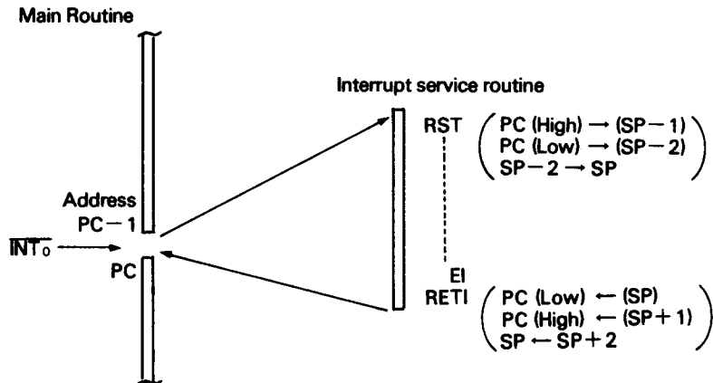
(a) \overline{\text{INT}}_0 Mode 0 Sequence when executing RST
