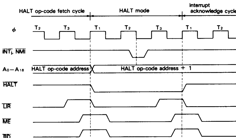
Figure 18 HALT Timing
