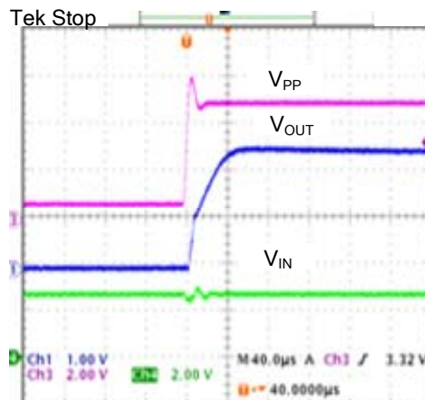
V_{PP} Start up Waveform
