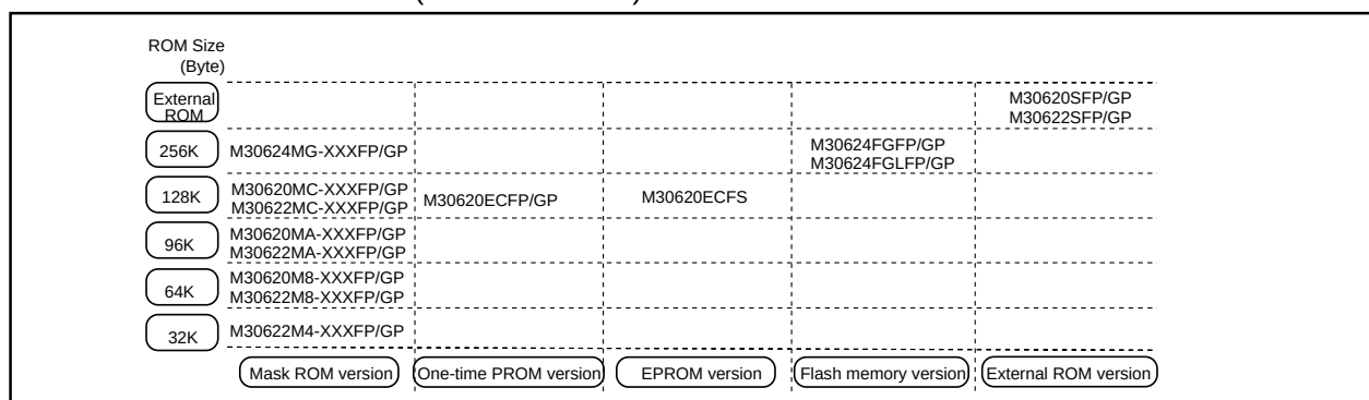
Figure 1.1.4. ROM expansion
