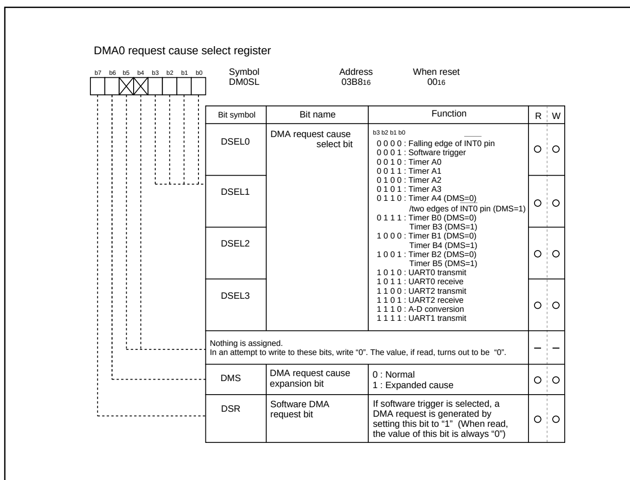
Figure 1.16.2. DMAC register (1)
