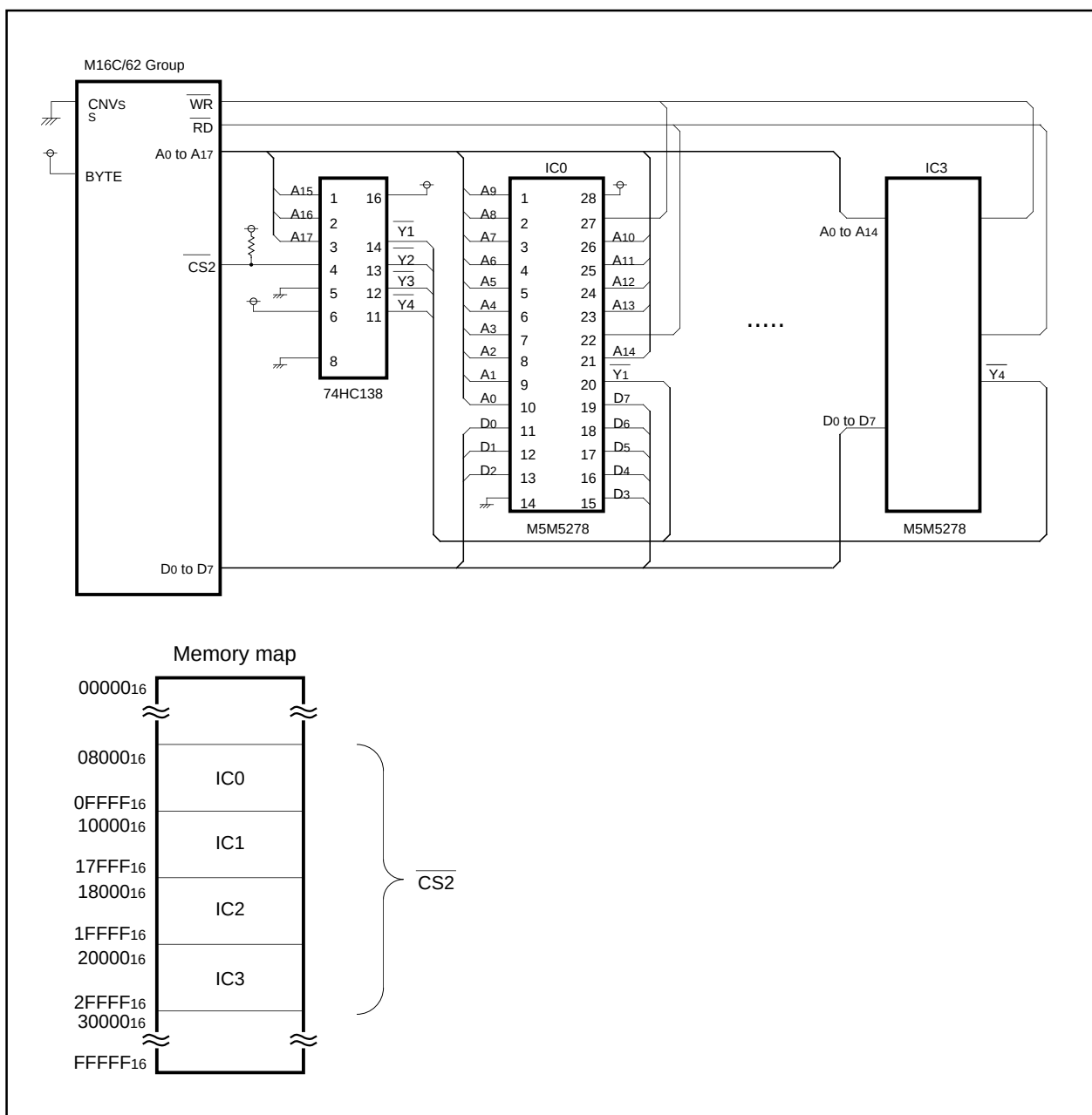
Figure 5.4.9. Chip selects and address bus
