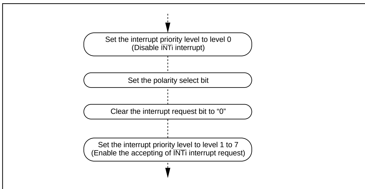
Figure 4.7.1. Switching condition of INT interrupt request
