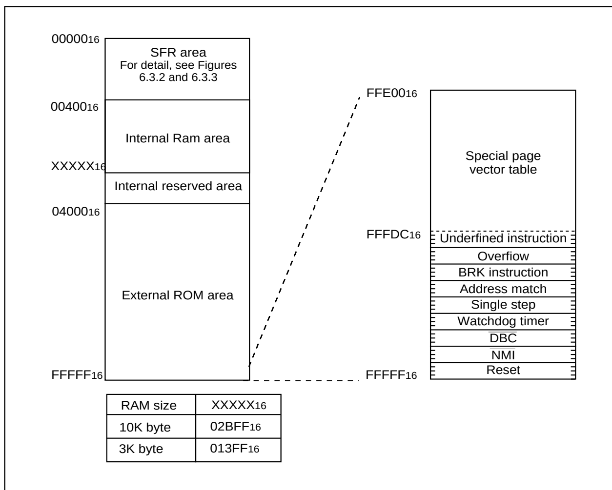
Figure 6.3.1. Memory map
