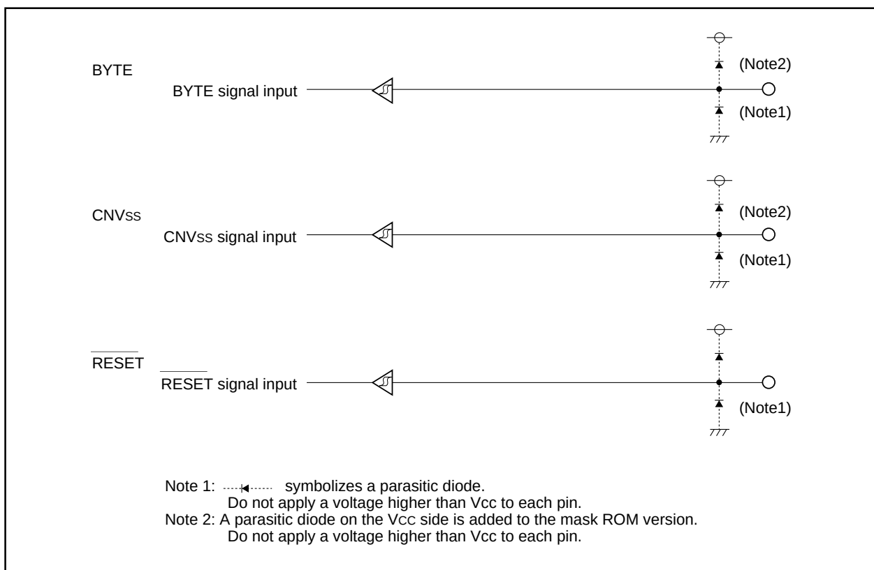
Figure 1.23.5. I/O pins
