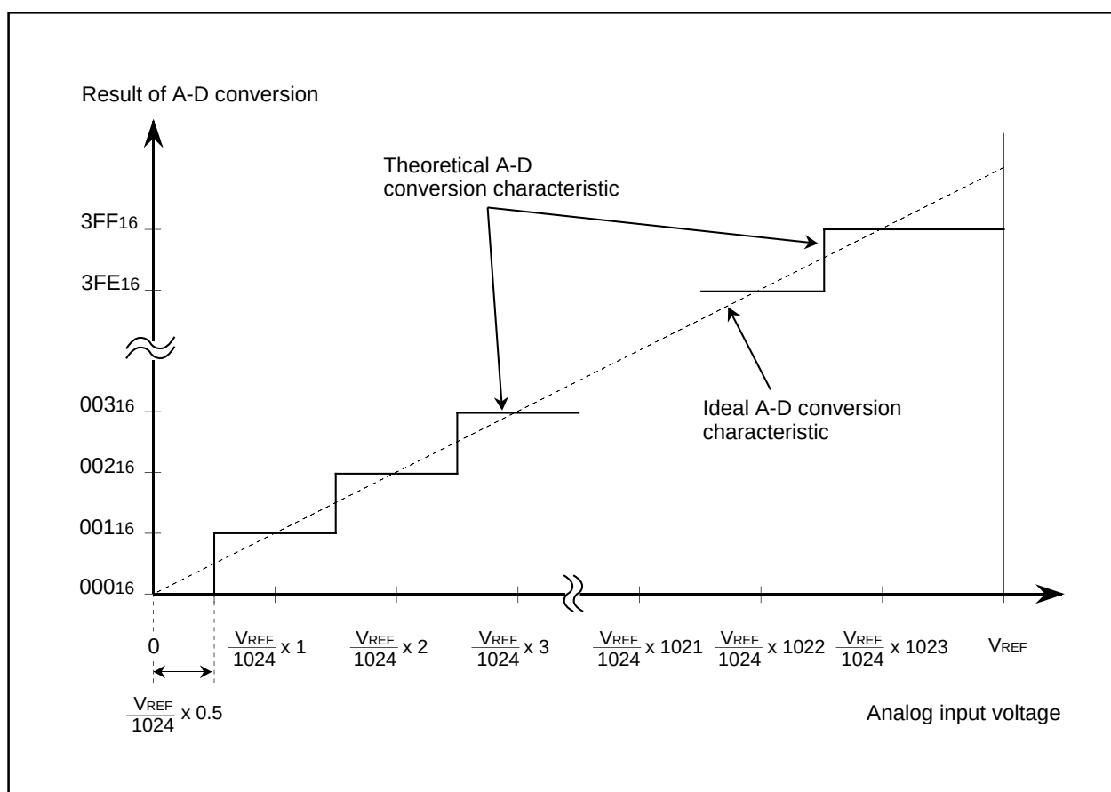
Figure 2.7.23. Theoretical A-D conversion characteristics (10-bit mode)
