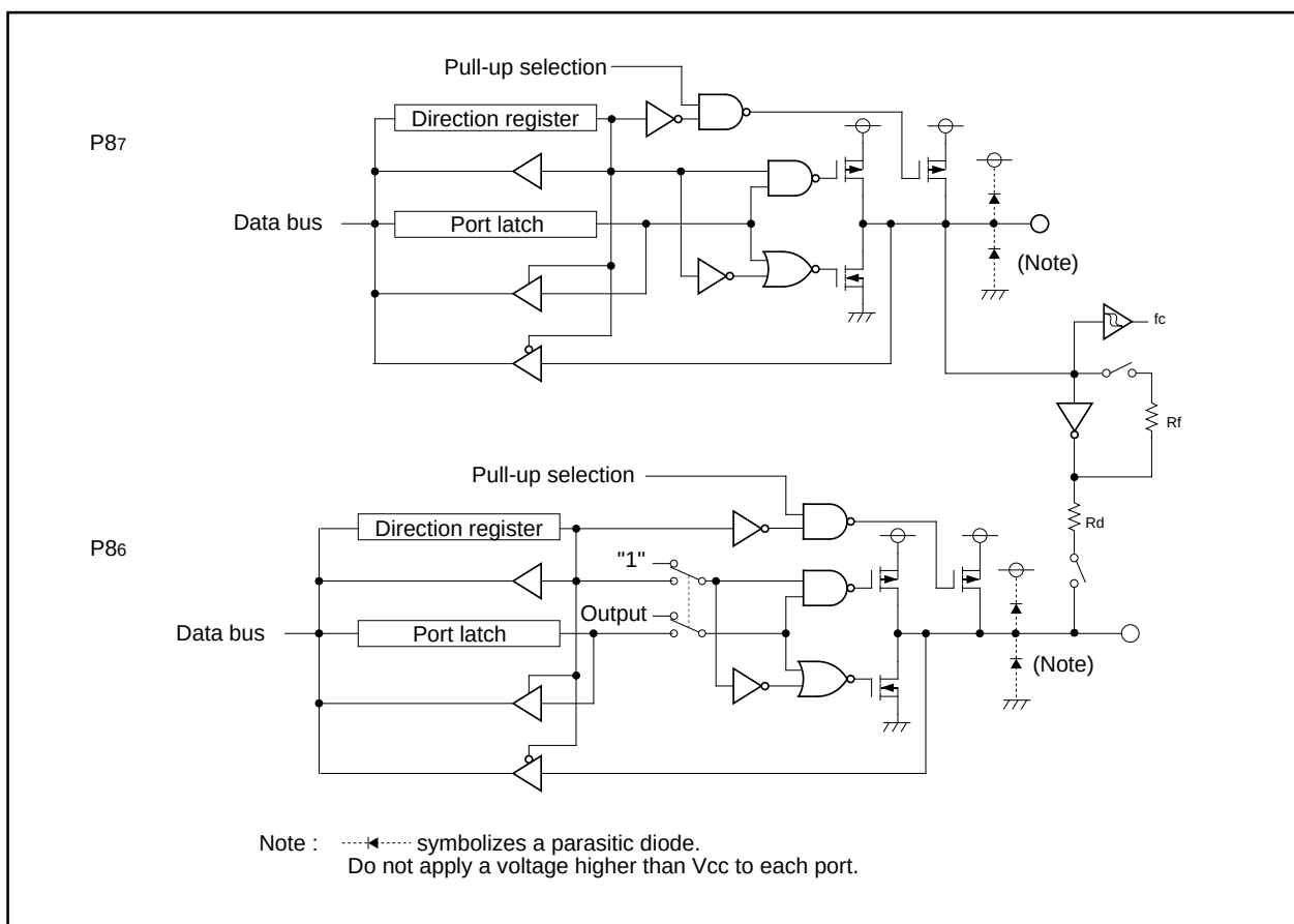
Figure 1.23.4. Programmable I/O ports (4)
