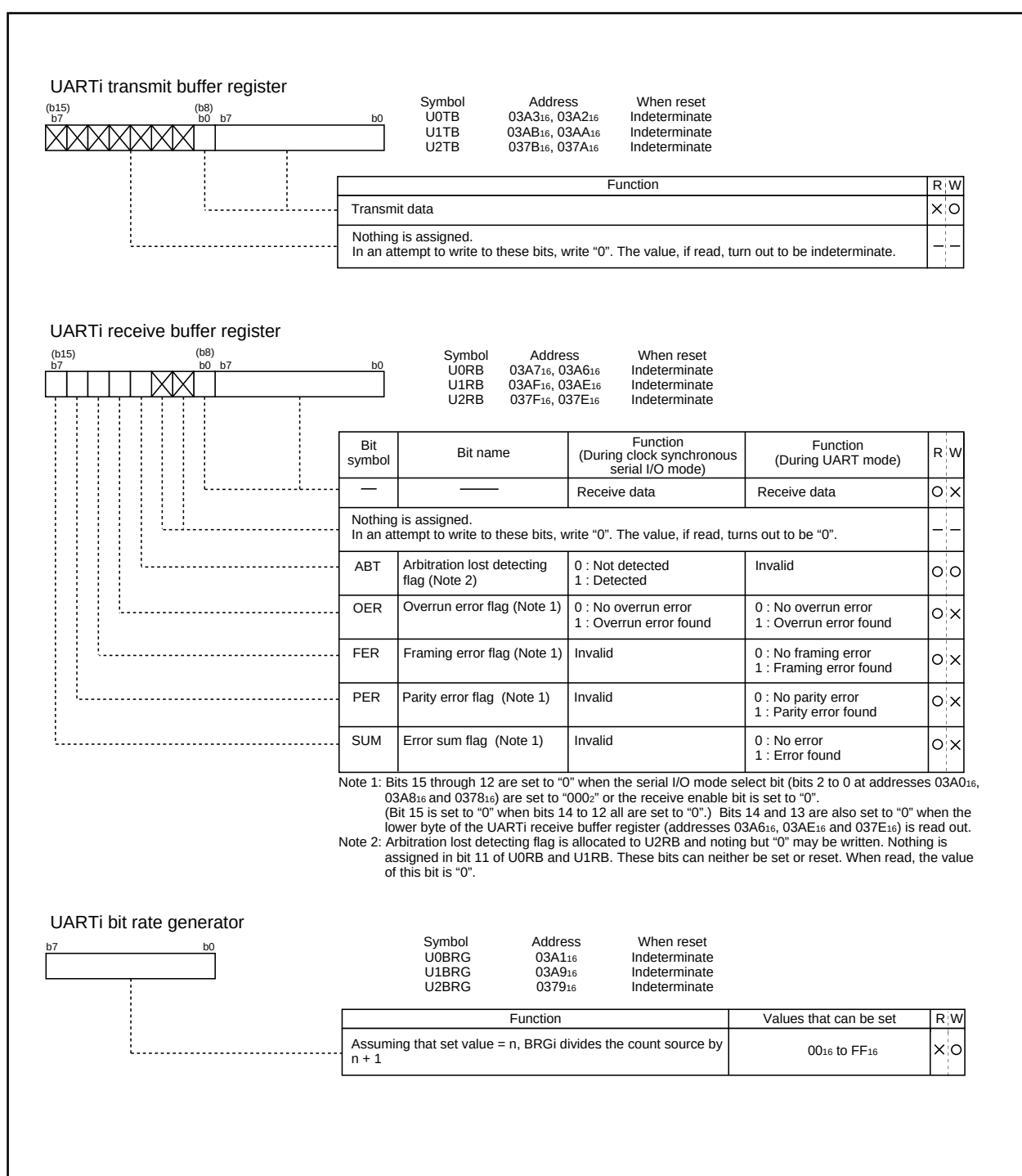
Figure 1.19.4. Serial I/O-related registers (1)
