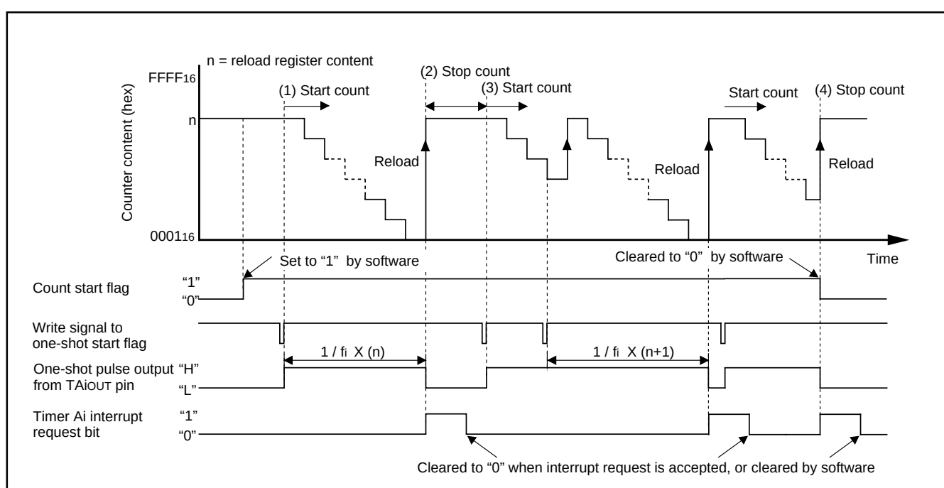
Figure 2.2.20. Operation timing of one-shot mode
