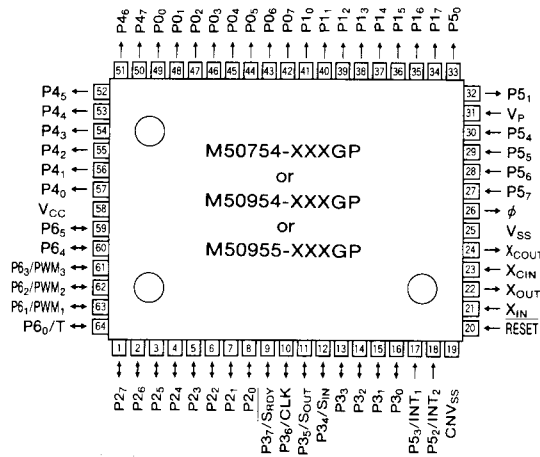
Outline 64P6W
