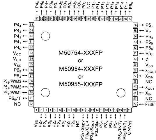
Outline 72P6
