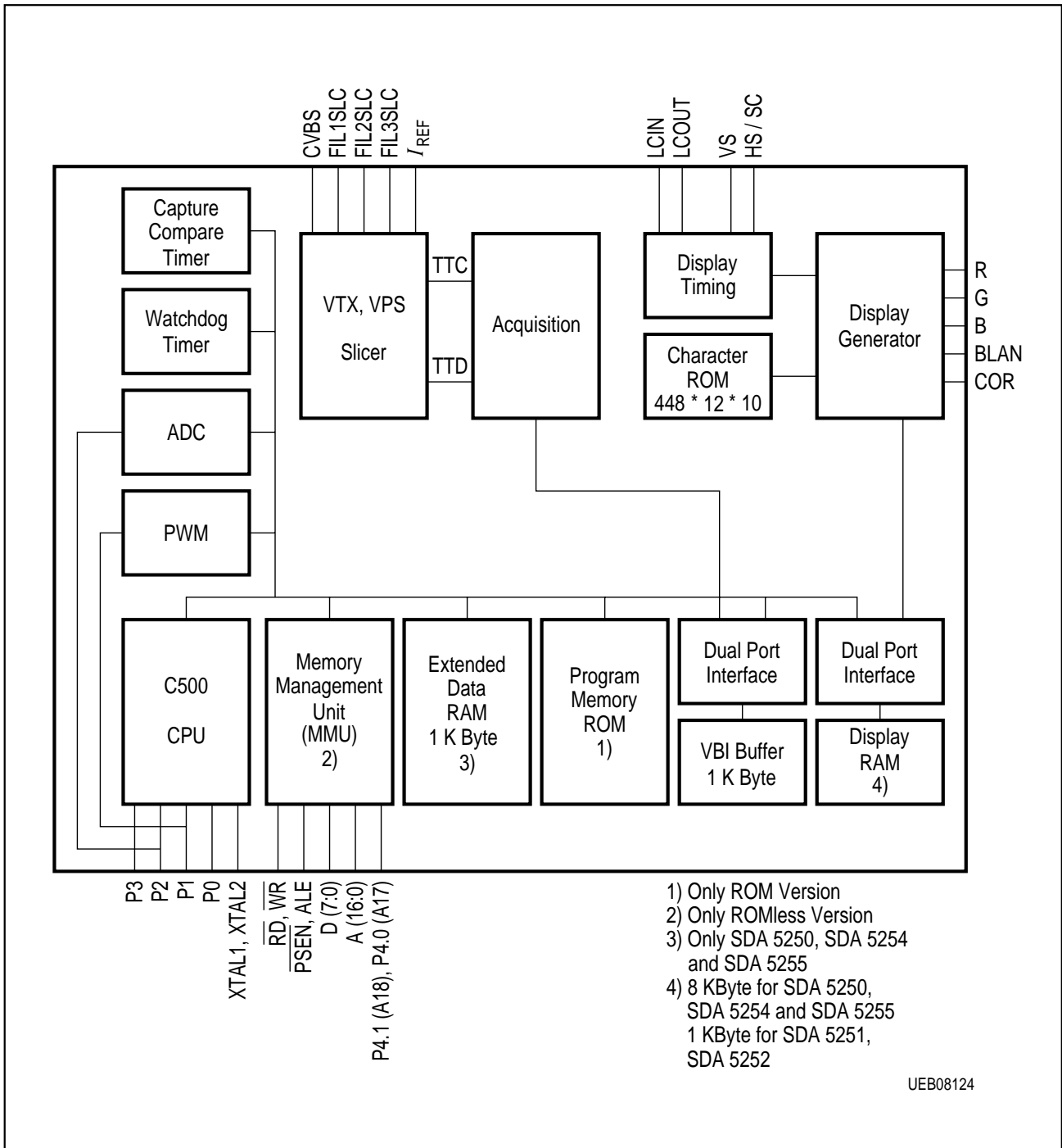
Figure 1 Block Diagram
