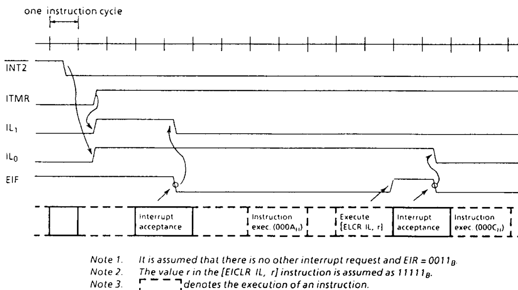
Figure 4-2. Interrupt Timing Chart (Example)
