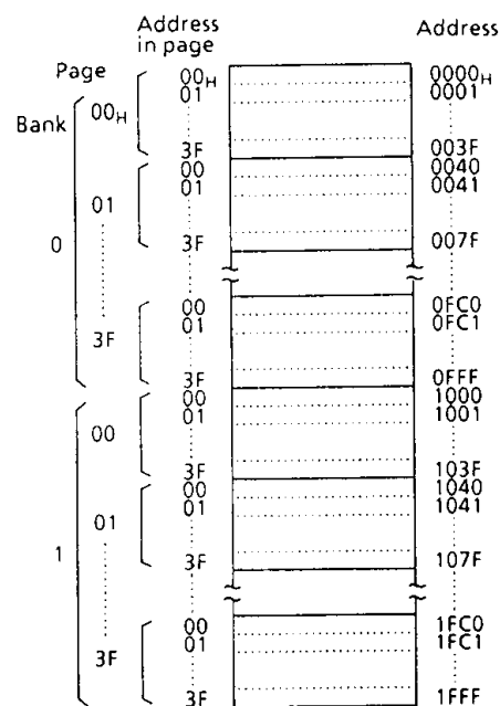
Figure 2-2. Configuration of Program Memory
