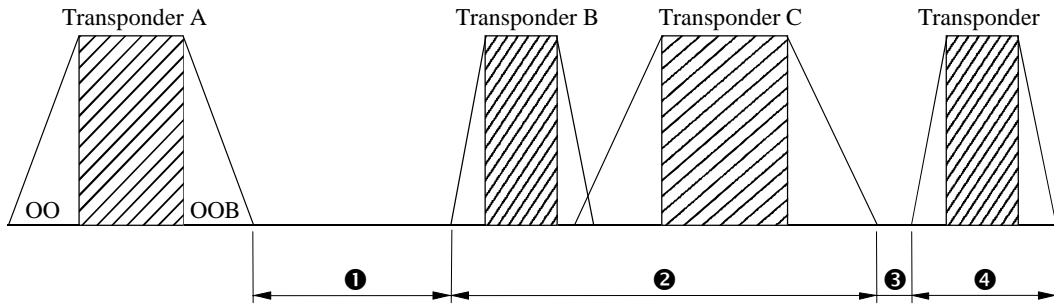
Figure 3.1. Example of the applicability of spurious emission limits
