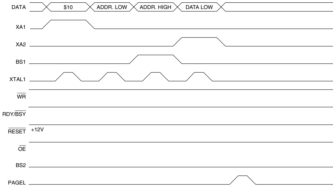
Figure 74. Programming the Flash Waveforms (Continued)
