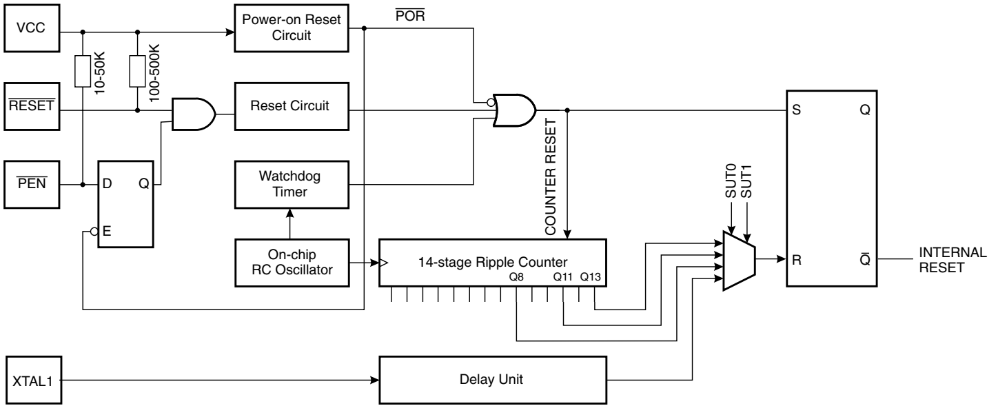
Figure 23. Reset Logic
