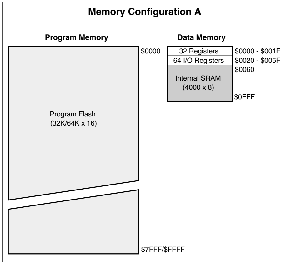
Figure 7. Memory Configurations
