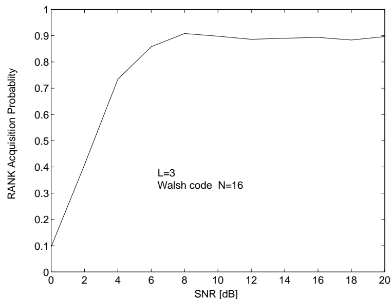
Figure 5.13: Correct rank acquisition probability in the context of MC-CDMA, when Walsh codes having a spreading factor of N = 16 were employed and K = 10 users were supported. BPSK transmission and an L = 3 -path Rayleigh fading channel were used. All system parameters are summarized in Table 5.3.
