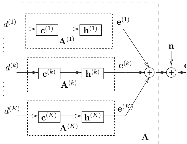
Figure 6.12: The DS-CDMA model for multipath channel
