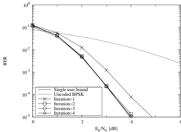
Figure 4.15: The PIC based iterative multiuser detector's BER versus E_b/N_0 performance, when communicating over a synchronous non-dispersive AWGN channel, while supporting K = 15 users. A \frac{1}{2} rate QPSK TTCM scheme having an effective throughput of 1 BPS was invoked.
