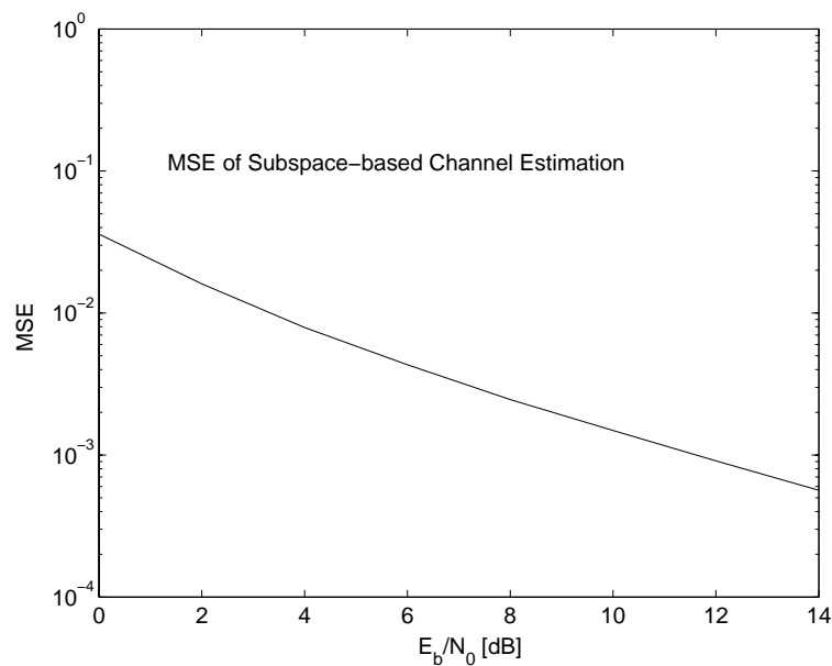
Figure 5.9: MSE performance of the subspace-based CIR estimator of the 3-element diversity receiver array aided DS-CDMA system using K = 10 , \tilde{K} = 7 , N = 15 .
