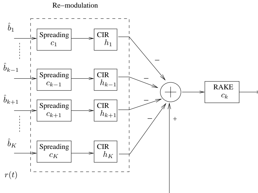
Figure 1.7: Schematic of the parallel interference canceller.
