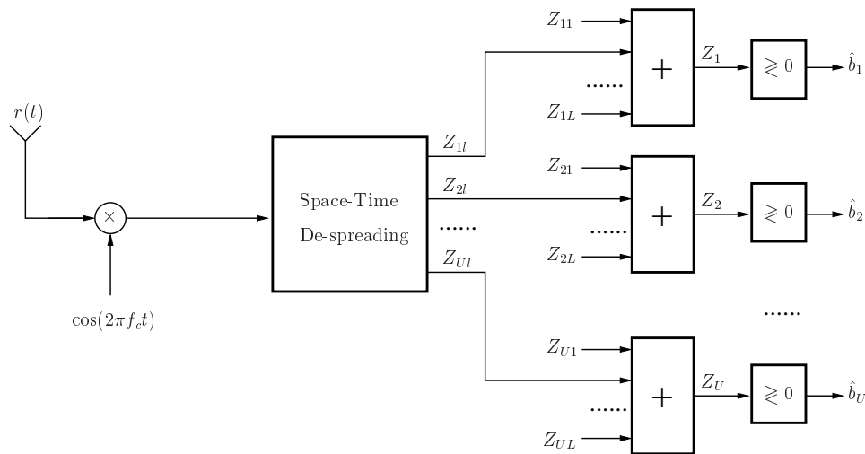
(b) Receiver
