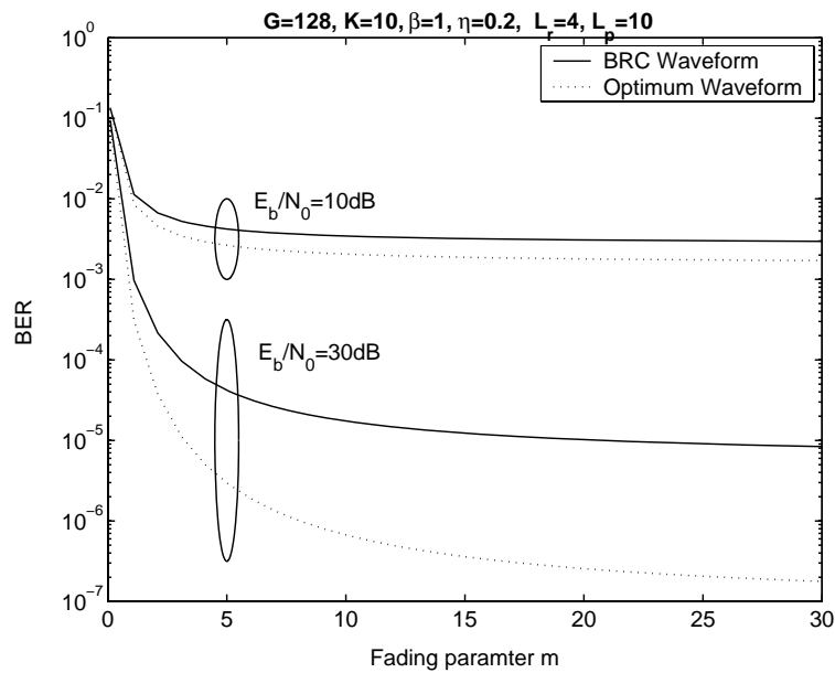
Figure 2.10: BER performance comparison of band-limited DS-CDMA as a function of the Nakagami fading parameter m in conjunction with the BRC and the optimum [23] waveforms, where the excess bandwidth was fixed to \beta = 1 , and the processing gain was G = 128 . A negative-exponentially decaying Multipath Intensity Profile (MIP) having a decay factor of \eta = 0.2 was used, the total number of resolvable paths was L_p = 10 , but the RAKE-receiver's complexity was limited to combining only L_r = 4 paths, and a total of K = 10 users were supported. As m increases, the channel becomes a dispersive AWGN-like transmission medium, resulting in a reduced BER.
