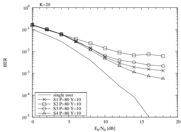
Figure 7.19: The GA assisted MC-CDMA MUD's BER performance, when communicating over asynchronous environments. The four different GA strategies listed in Table 7.2 were adopted for approaching the optimum MUD's performance and the number of users supported was K = 20 . The population size was P = 80 and the number of generations was Y = 10 . Furthermore, the number of subcarriers was M = 4 and each subcarrier experienced uncorrelated narrowband Rayleigh fading.
