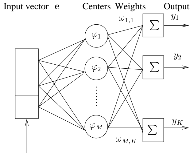
Figure 6.10: The architecture of RBF based MUD.
