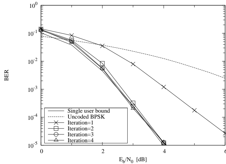
Figure 4.16: The PIC based iterative multiuser detector's BER versus E_b/N_0 performance, when communicating over an asynchronous non-dispersive AWGN channel, while supporting K = 7 users. A \frac{1}{2} rate QPSK TCM scheme having an effective throughput of 1 BPS was invoked.
