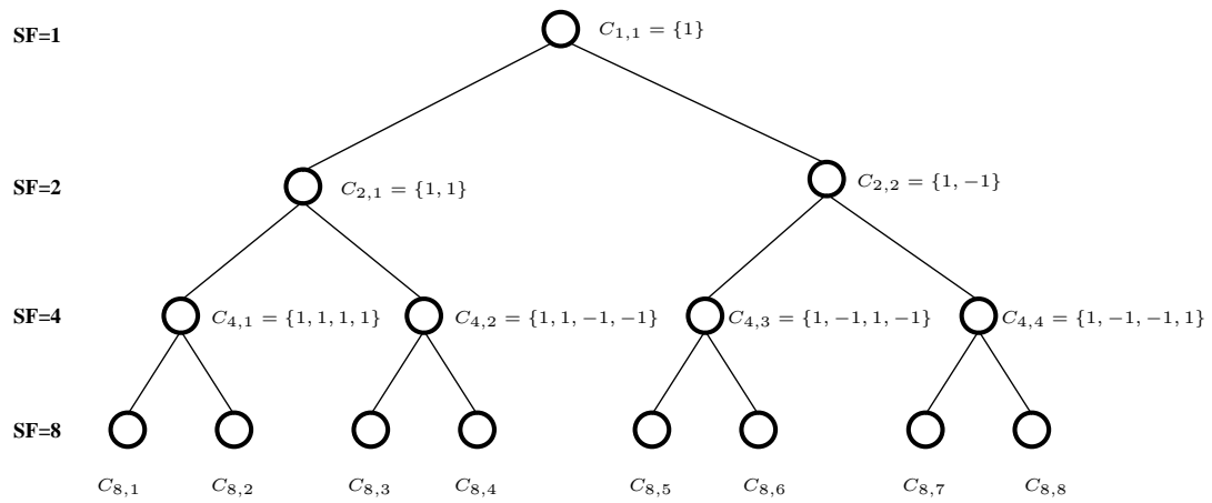
Figure 9.1: Tree structure of the OVSF spreading codes.
