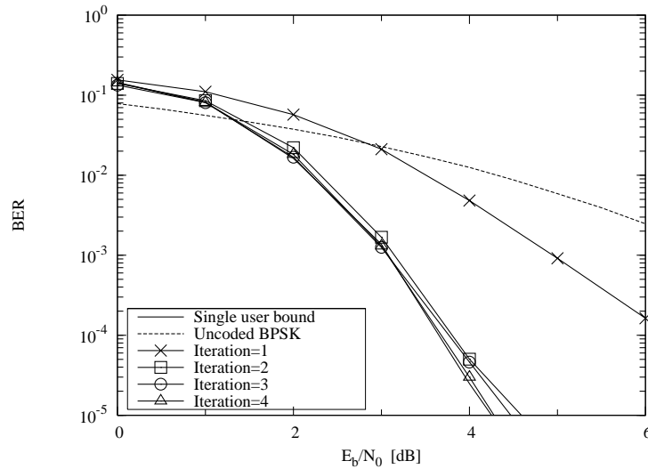
Figure 4.26: The PIC based iterative multiuser detector's BER performance, when communicating over a asynchronous non-dispersive AWGN channel, while supporting K = 7 users. A \frac{1}{2} -rate LDPC was invoked as well as QPSK modulation was employed.
