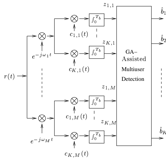
Figure 7.2: Schematic of the GA assisted MUD aided MC-CDMA base station receiver
