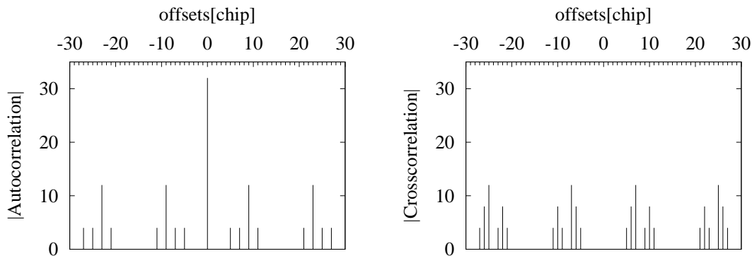
(a) Autocorrelation
