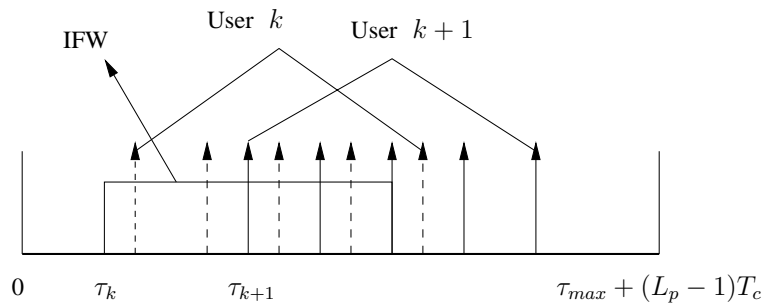
Figure 3.5: Illustration of the interference suppression capability of the LAS codes for the first finger of the RAKE receiver, when the width of the IFW is \iota = 2 .
