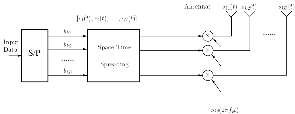
(a) Transmitter
