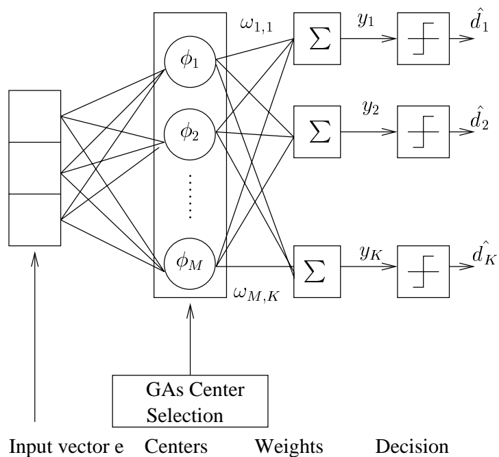
Figure 6.13: Structure of GA-RBF assisted MUD
