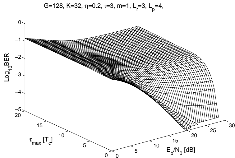
Figure 3.12: BER performance of LAS CDMA as a function of the maximum delay difference \tau_{max} and E_b/N_0 , when communicating over a Rayleigh fading channel having m = 1 . K = 32 users were supported. The negative exponential MIP decay factor was \eta = 0.2 , the IFW width was \iota = 3 , and the number of resolvable paths was L_p = 4 . The RAKE receiver combined L_r = 3 paths.
