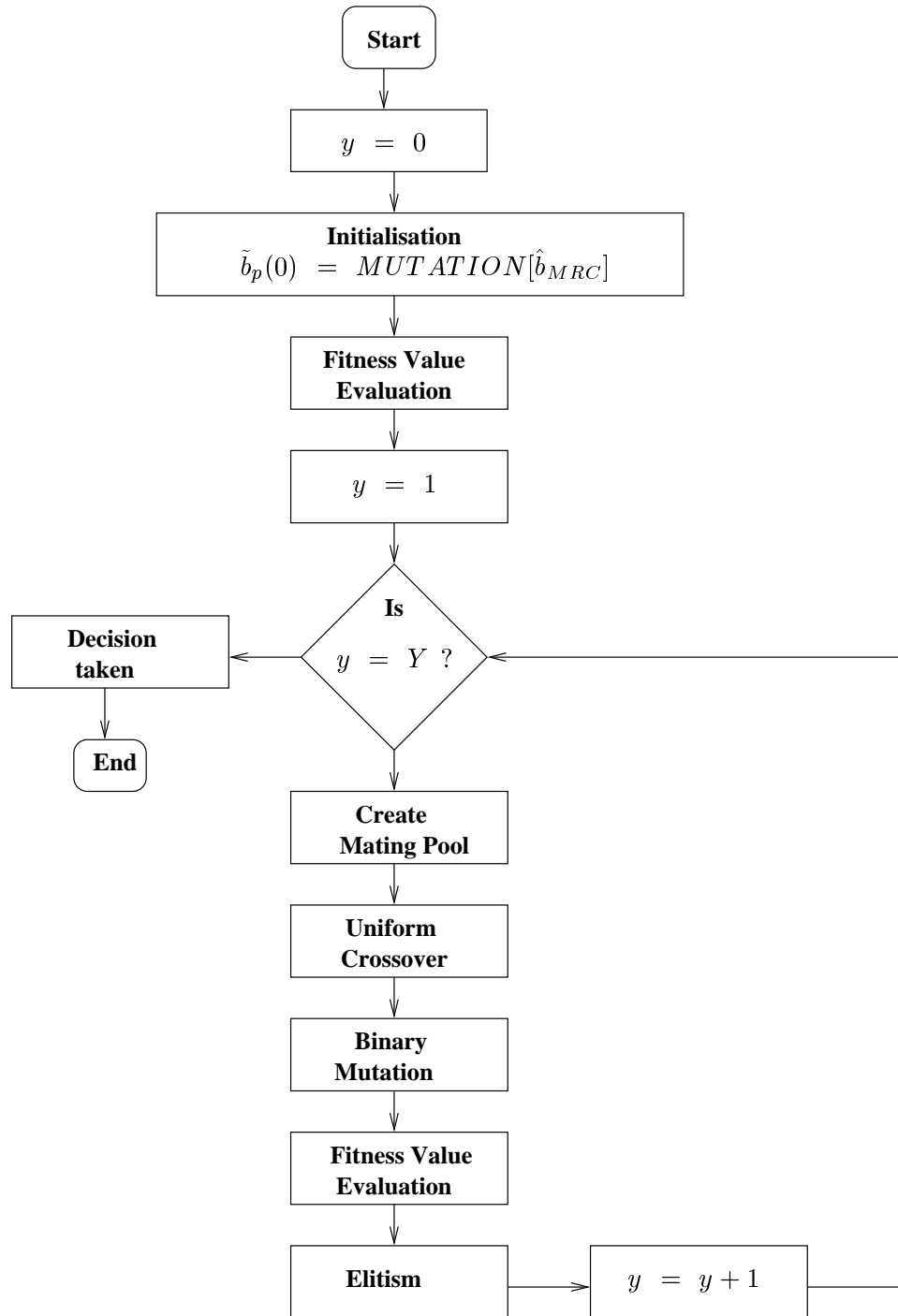
Figure 7.3: A flowchart depicting the structure of a genetic algorithm assisted MUD in the context of the synchronous MC-CDMA base station receiver
