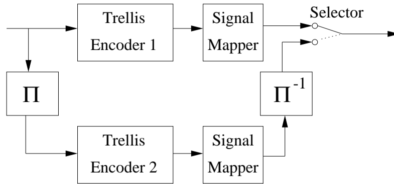
Figure 4.1: Turbo trellis-coded modulation encoder.
