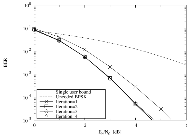
Figure 4.8: The PIC based iterative multiuser detector's BER versus E_b/N_0 performance, when communicating over a synchronous non-dispersive AWGN channel, while supporting K = 15 users. A \frac{1}{2} rate QPSK TCM scheme having an effective throughput of 1 BPS was invoked.
