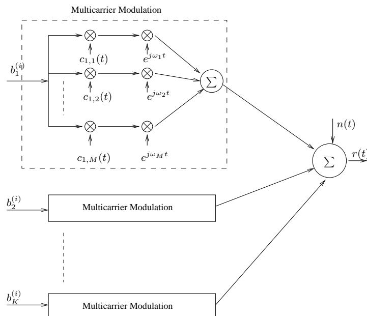
Figure 7.1: The transmitter of a MC-CDMA system
