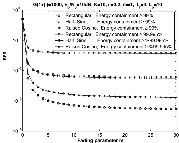
Figure 2.7: BER performance comparisons of various band-limited DS-CDMA systems as a function of the Nakagami fading parameter m in conjunction with three time-limited chip-waveforms, where two different energy containment factors, namely \geq 99\% and \geq 99.995\% were considered. A negative-exponentially decaying Multipath Intensity Profile (MIP) having a decay factor of \eta = 0.2 was used, the total number of resolvable paths was L_p = 10 , but the RAKE-receiver's complexity was limited to combining only L_r = 4 paths. A total of K = 10 users were supported.
