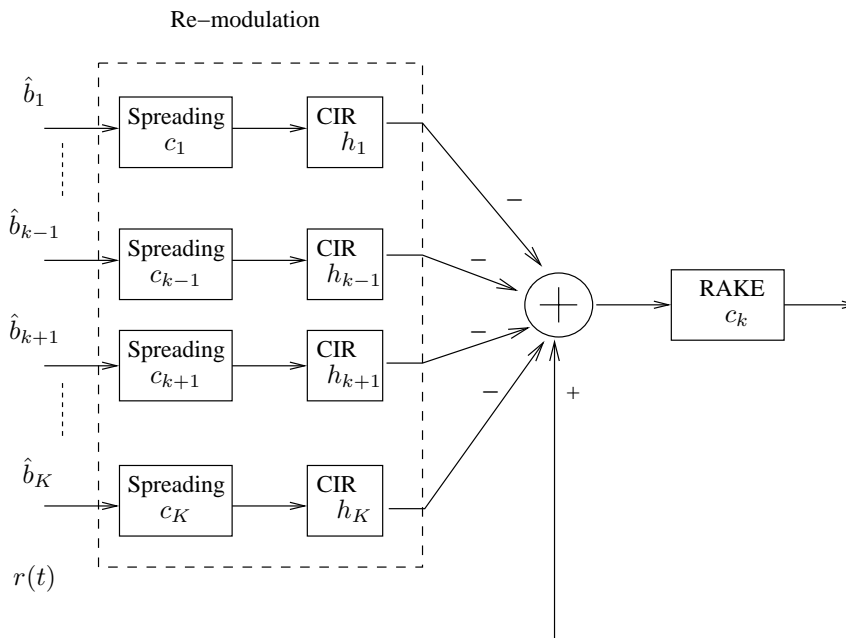
Figure 4.3: Schematic of a single PIC stage.
