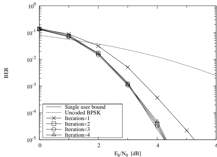
Figure 4.25: The PIC based iterative multiuser detector's BER performance, when communicating over a synchronous non-dispersive AWGN channel, while supporting K = 15 users. A \frac{1}{2} -rate LDPC was invoked as well as QPSK modulation was employed.
