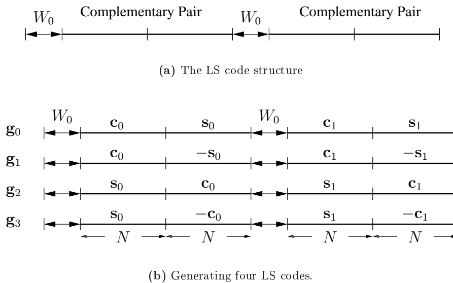
Figure 3.2: Generating the LS(N, P, W_0) code using the (P \times P) = (4 \times 4) Walsh-Hadamard matrix components (1, 1, 1, 1) and (1, -1, 1, -1) .
