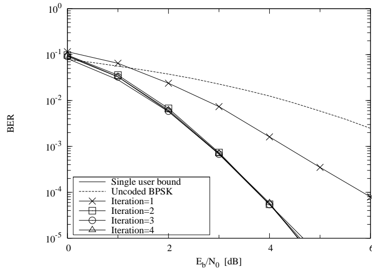
Figure 4.9: The PIC based iterative multiuser detector's BER versus E_b/N_0 performance, when communicating over an asynchronous non-dispersive AWGN channel, while supporting K = 7 users. A \frac{1}{2} rate QPSK TCM scheme having an effective throughput of 1 BPS was invoked.
