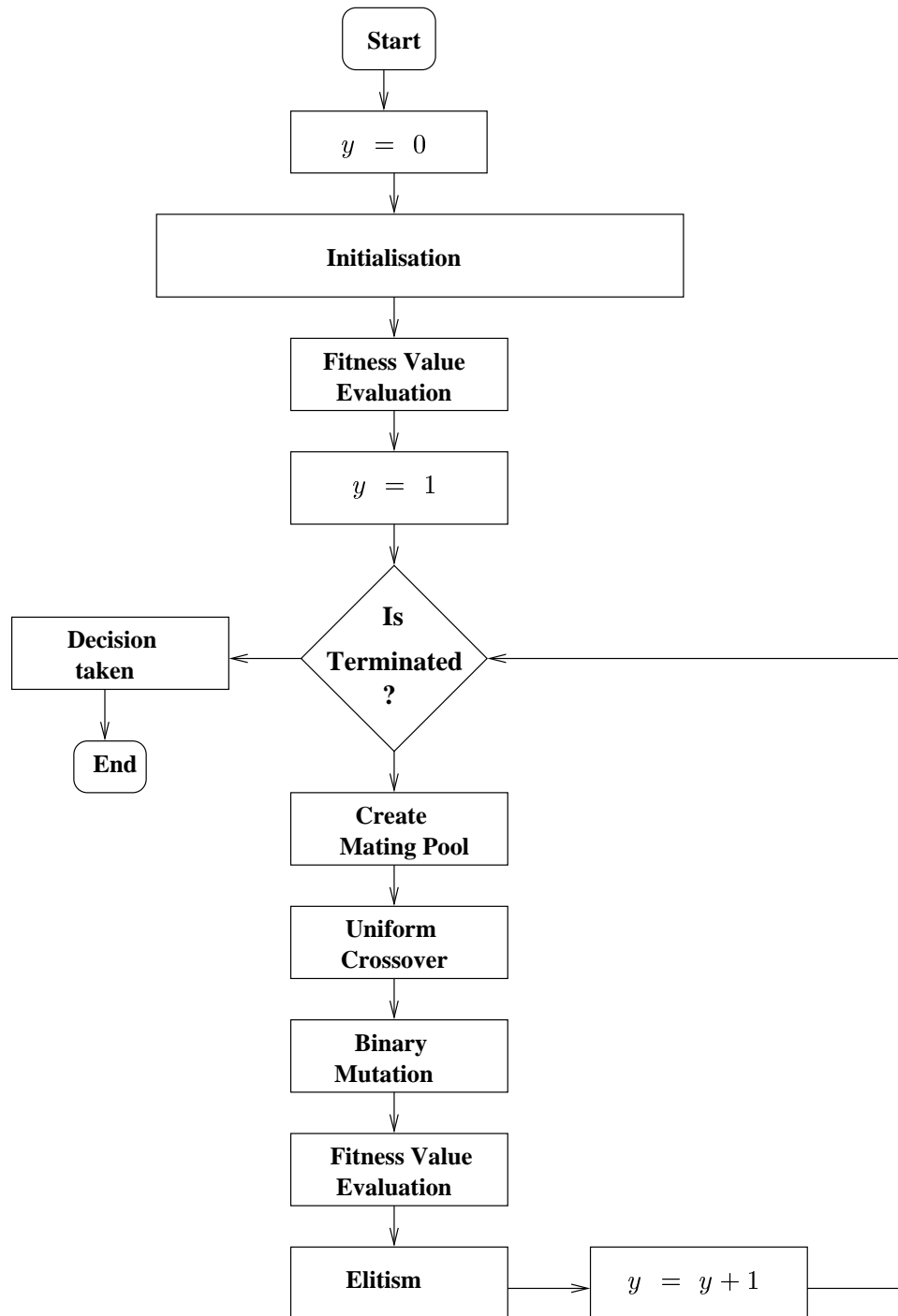
Figure 1.8: Flowchart of a GA-based multiuser detector.
