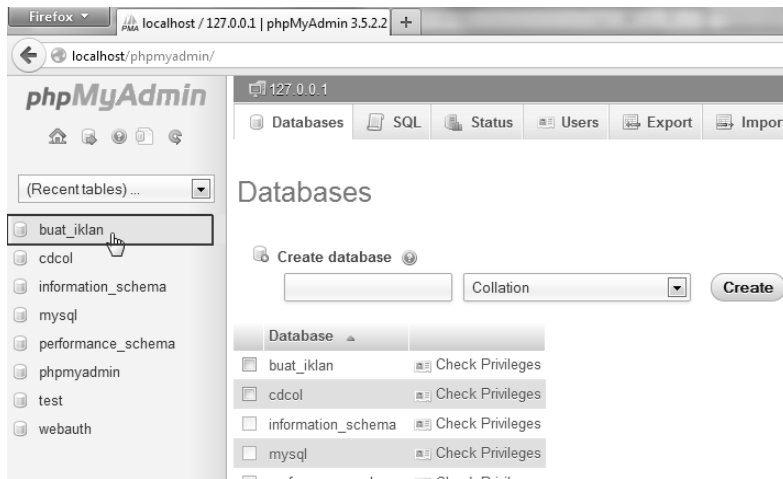
Gambar 1.10 Laman PHPMyAdmin
