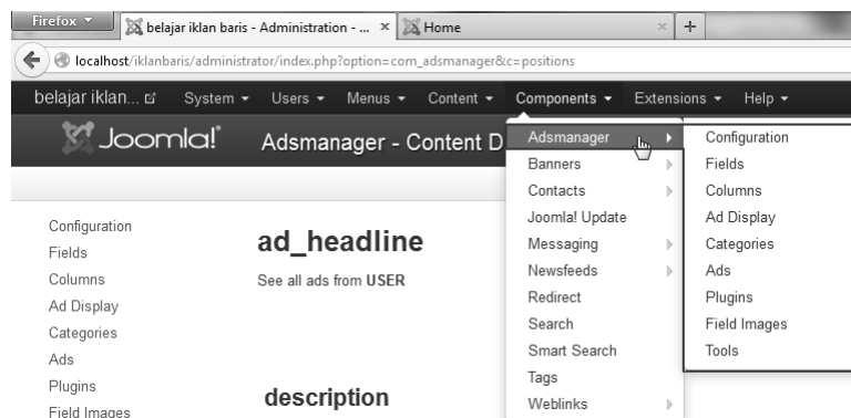
Gambar 1.38 Menu AdsManager
