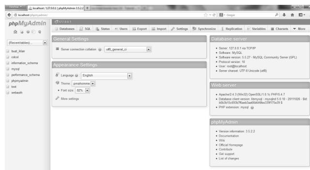
Gambar 1.8 Laman PHPMYAdmin
