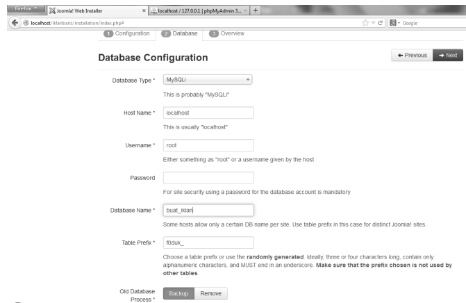
Gambar 1.24 Database Configuration
