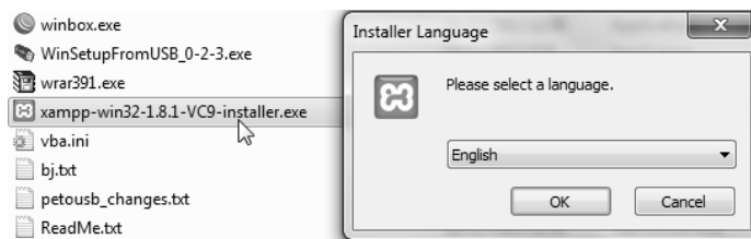
Gambar 1.11 File xampp-win32-1.8.1-vc9-installer.exe
