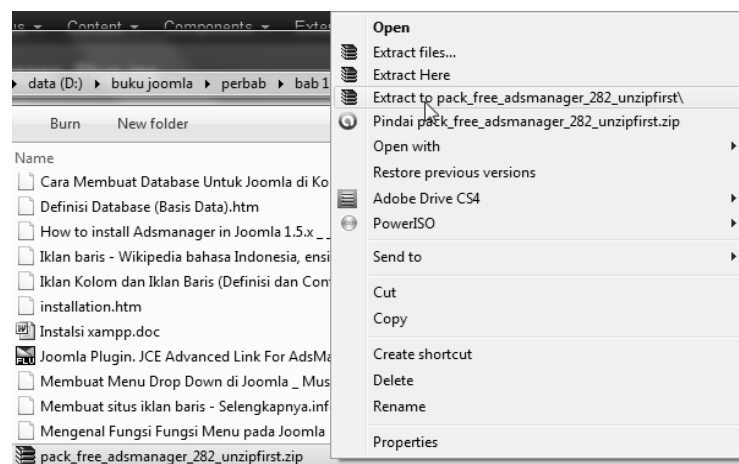
Gambar 1.32 AdsManager Packet
