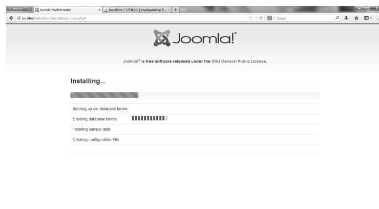
Gambar 1.27 Proses instalasi
