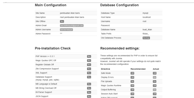
Gambar 1.26 Laman Overview
