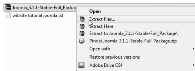
Gambar 1.20 Extract Joomla
