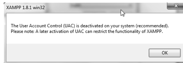
Gambar 1.12 Warning UAC
