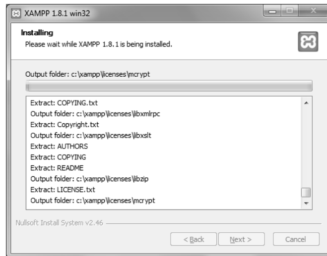
Gambar 1.15 Proses instalasi
